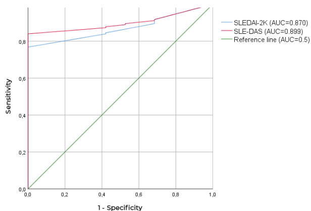
Figure 1. ROC curves for SLE-DAS and SLEDAI-2K using DORIS criteria as the reference standard
