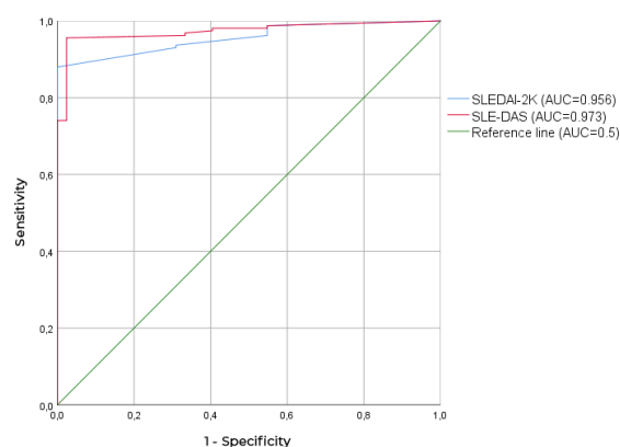
Figure 2. ROC curves for SLE-DAS and SLEDAI-2K using DORIS criteria as the reference standard excluding glucocorticoid dose
